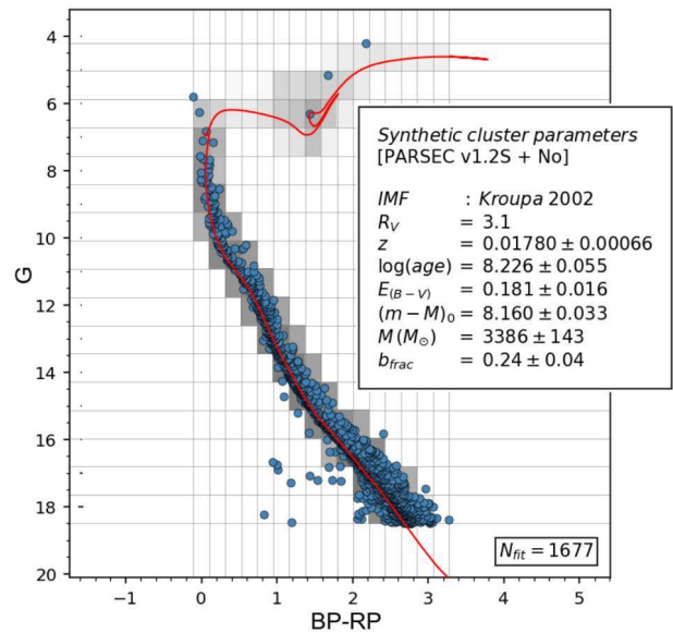
Figure 3: Fundamental parameters estimated by ASTECA for the NGC 2516 open cluster. N_{fit} is the number of members stars used in the analysis.
