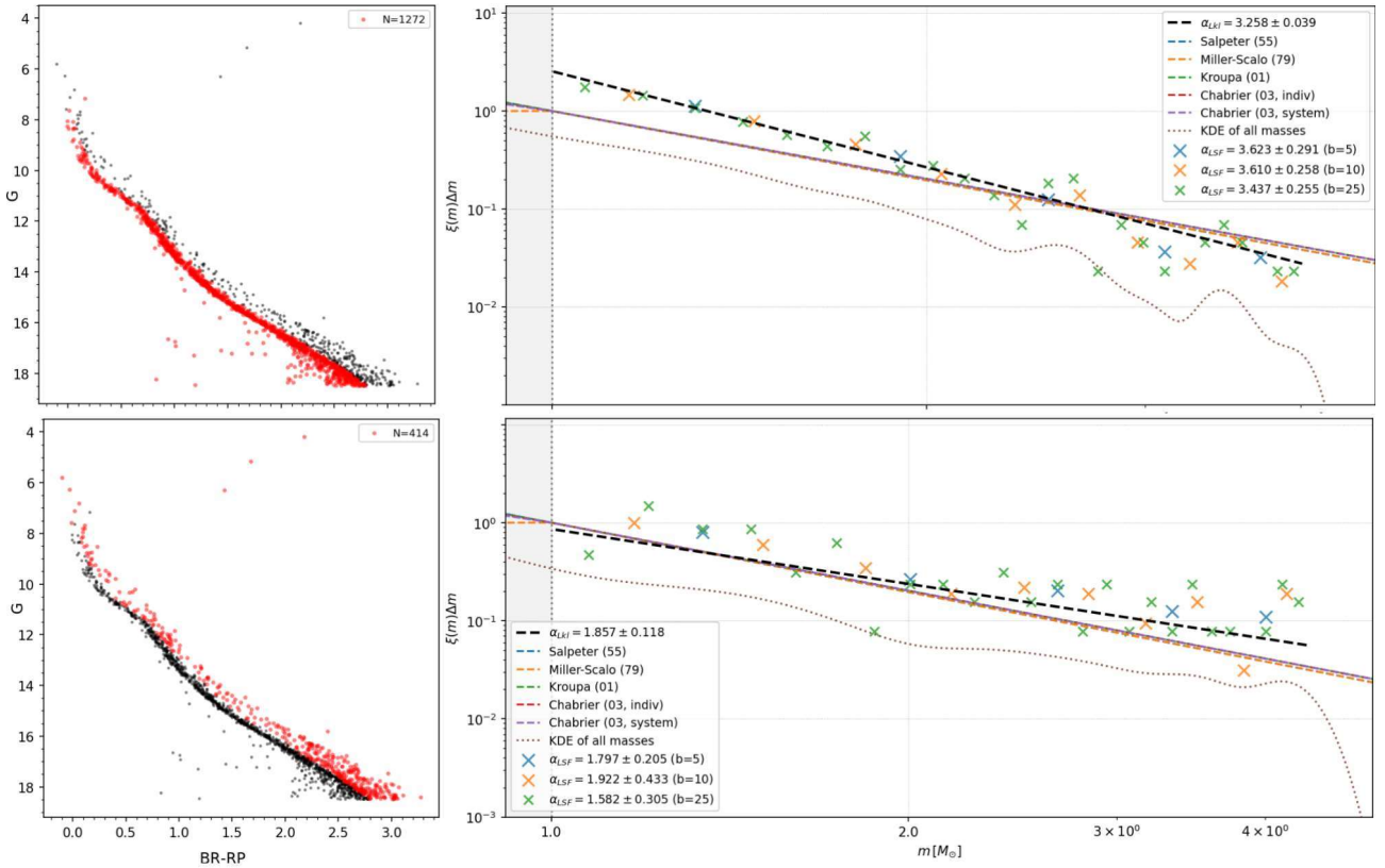
Figure 4: Estimation of the IMF for NGC 2516. Top left : CMD with the main sequence in red. Top right : IMF for the main sequence as a black dashed line. Bottom left : CMD with the binary sequence in red. Bottom right : IMF for the binary sequence as a black dashed line. Colored dashed lines represent several published IMFs. Colored crosses are least square fits (LSF) obtained using histograms with 5, 10, and 25 mass bins.
