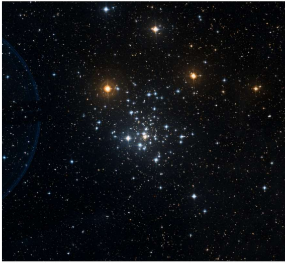
Figure 1: A 60x53 arcmin image of the central part of NGC 2516. North is up, East to the left.
