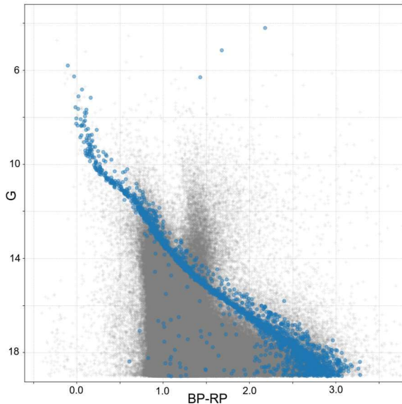
Figure 2: Color-magnitude diagram (CMD) of NGC 2516. Members estimated with PYUPMASK are shown in blue, field stars are shown in grey.
