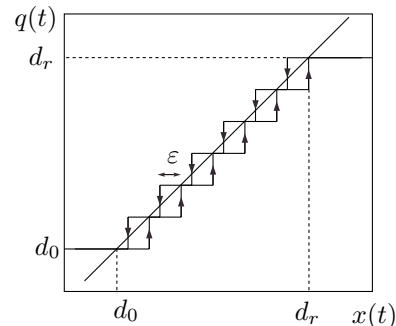
Figure 1: Quantization Function with hysteresis
