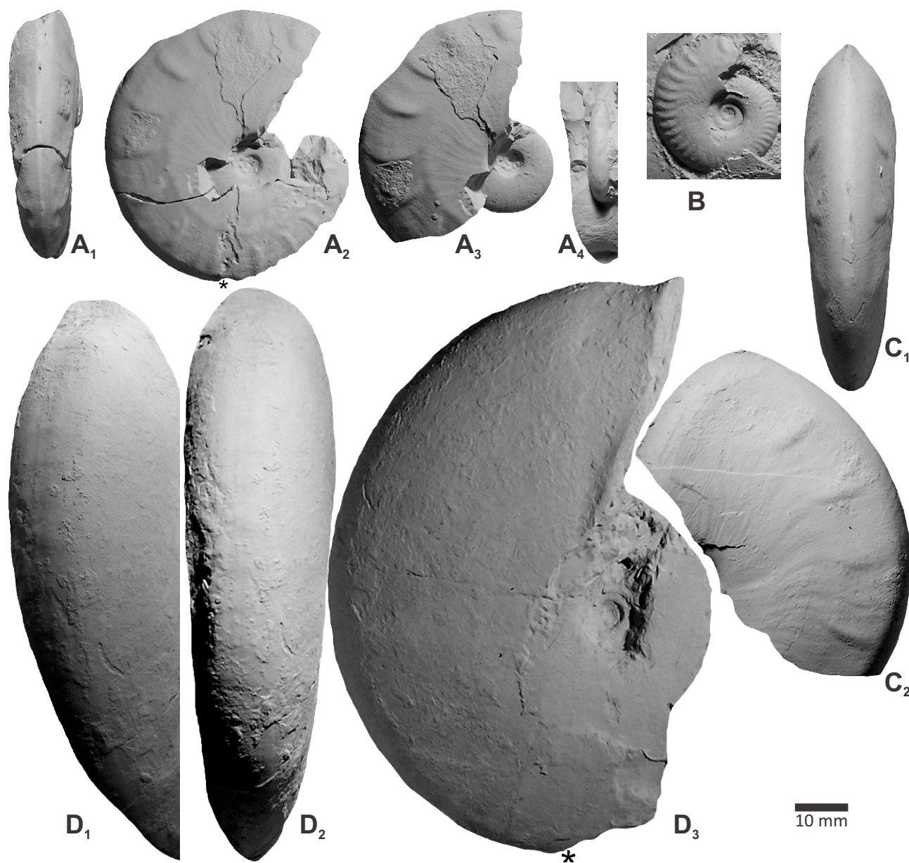
Figure 8. A-B: Alcidellus aff. obsoletooides Riccardi, Westermann & Elmi, 1989, level CM-3, Steinmanni Subzone, Steinmanni Zone. A: complete adult macroconch (MOZ-PI-7412/1); ventral (A 1 ) and lateral (A 2 ) views, A 3 : lateral view with last part of the phragmocone removed showing the inner whorls, A 4 : ventral view of the inner whorls. B: adult macroconch phragmocone (MOZ-PI-7412/3). C-D: Alcidellus n. sp. aff. tenuistriatus (Grossouvre, 1888), level CM-35, Gerthi Subzone, Steinmanni Zone. C: adult macroconch beginning of bodychamber (MOZ-PI-7430/4), C 1 : ventral view showing a weak tricarination, C 2 : lateral view showing distant lunuloid ribs on the upper flank. D: adult macroconch with peristome (MOZ-PI-7430/7); D 1 -D 2 : ventro-lateral and ventral views of the bodychamber showing ventral tabulation; D 3 : lateral view, note the wide and shallow constriction preceding the flared peristome. —All natural size (x1). Asterisk at last septum.
