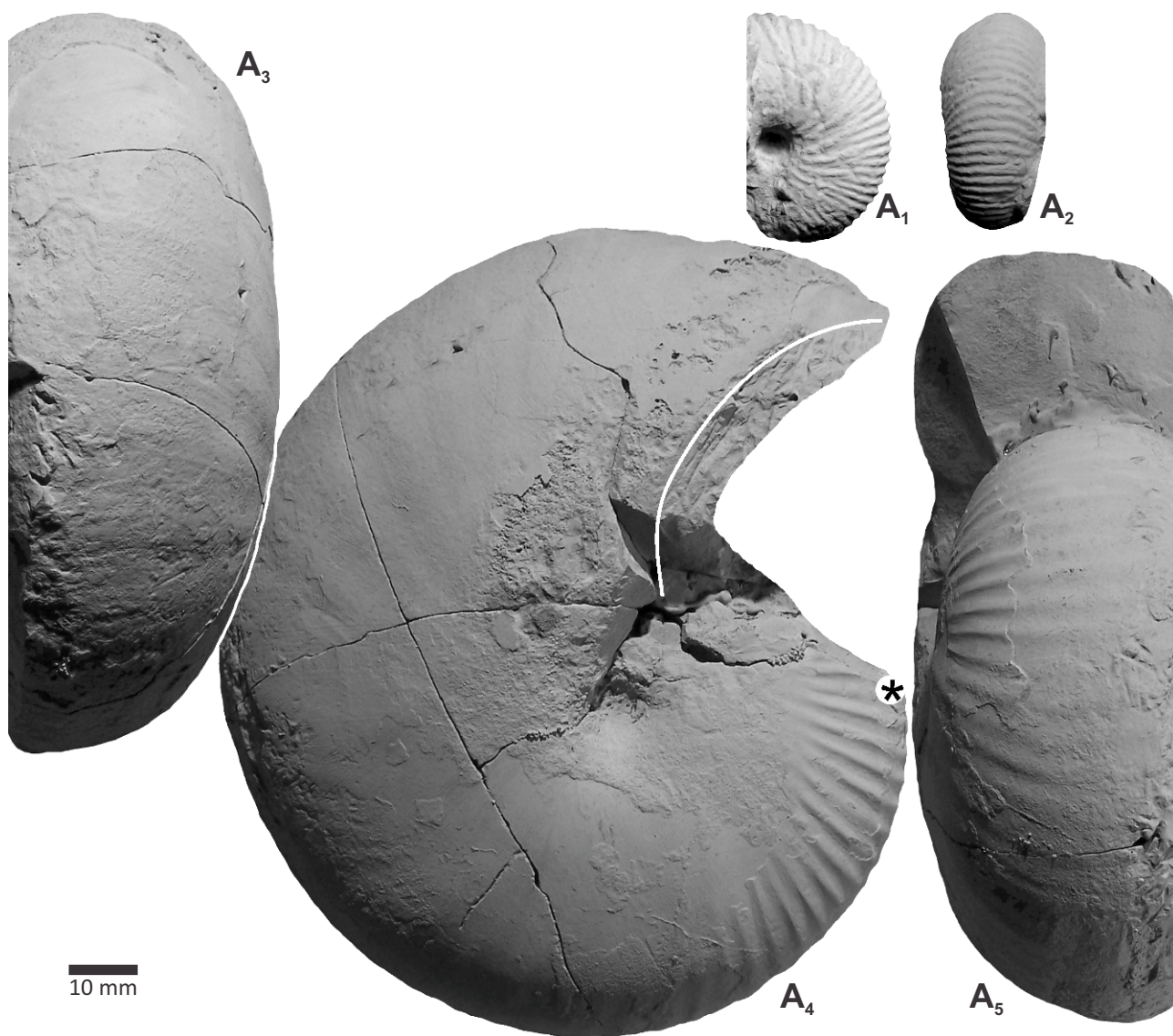
Figure 22. Lilloettia australis Riccardi & Westermann, 1991a, level CM-6b, crassus Hz., Gerthi Subzone, Steinmanni Zone. Complete adult macroconch (MOZ-PI-7416); A 1 -A 2 : inner whorls; A 3 : ventral view of the bodychamber showing wide, blunt ribbing vanishing towards the peristome; A 4 : lateral view; A 5 : apertural view. – All natural size (x1). Asterisk at last septum.
