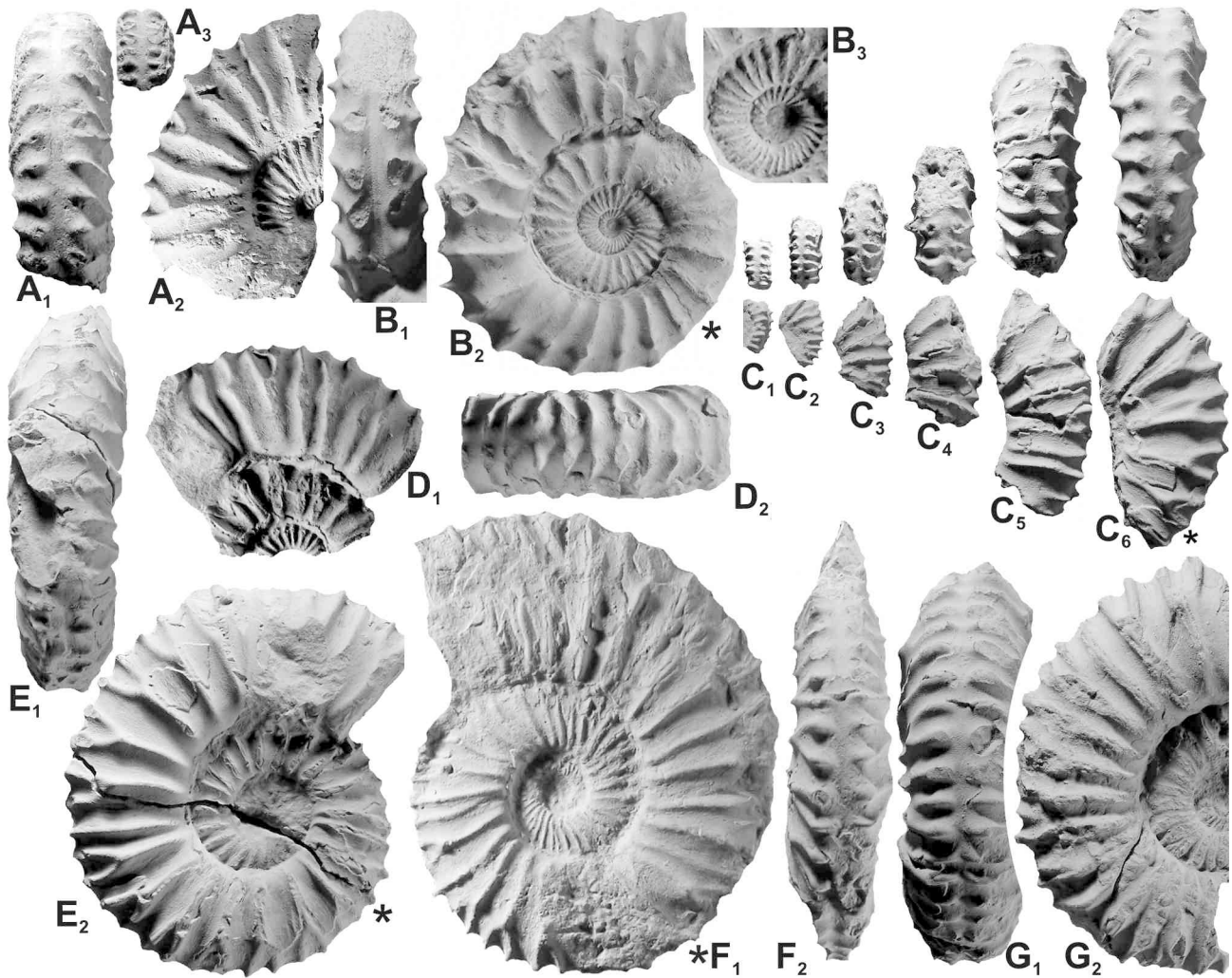
Figure 34. Corongoceras mendozanum (Behrendsen). A. Cieneguita, beds AC-14 and AC-15 (Alternans Zone). A: incomplete ?macroconch phragmocone (MCNAM 24459); A 2 : detail of the venter of the penultimate whorl. B: complete adult microconch with lappets (MCNAM 24458/1); B 2 : detail of the innermost whorls (x2). C: juvenil macroconch dissected for showing the ontogeny in ventral (upper row) and corresponding lateral (lower row) views (MCNAM 24459/24) at about D = 8-10 mm (C 1 ), D = 13 mm (C 2 ), D = 20 mm (C 3 ), D = 25 mm (C 4 ), D = 35 mm (C 5 ) and D = 41 mm (C 6 , bodychamber). D: adult microconch with lappets (MCNAM 24459/11). E: macroconch with incomplete bodychamber (MCNAM 24459/2). F: adult macroconch with incomplete bodychamber (MCNAM 24459/4), compressed variant. G: macroconch phragmocone with incomplete bodychamber (MCNAM 24459/2), stout variant. All natural size except E 2 (x2). All natural size (x1) otherwise indicated. Asterisk indicating the last septum.
