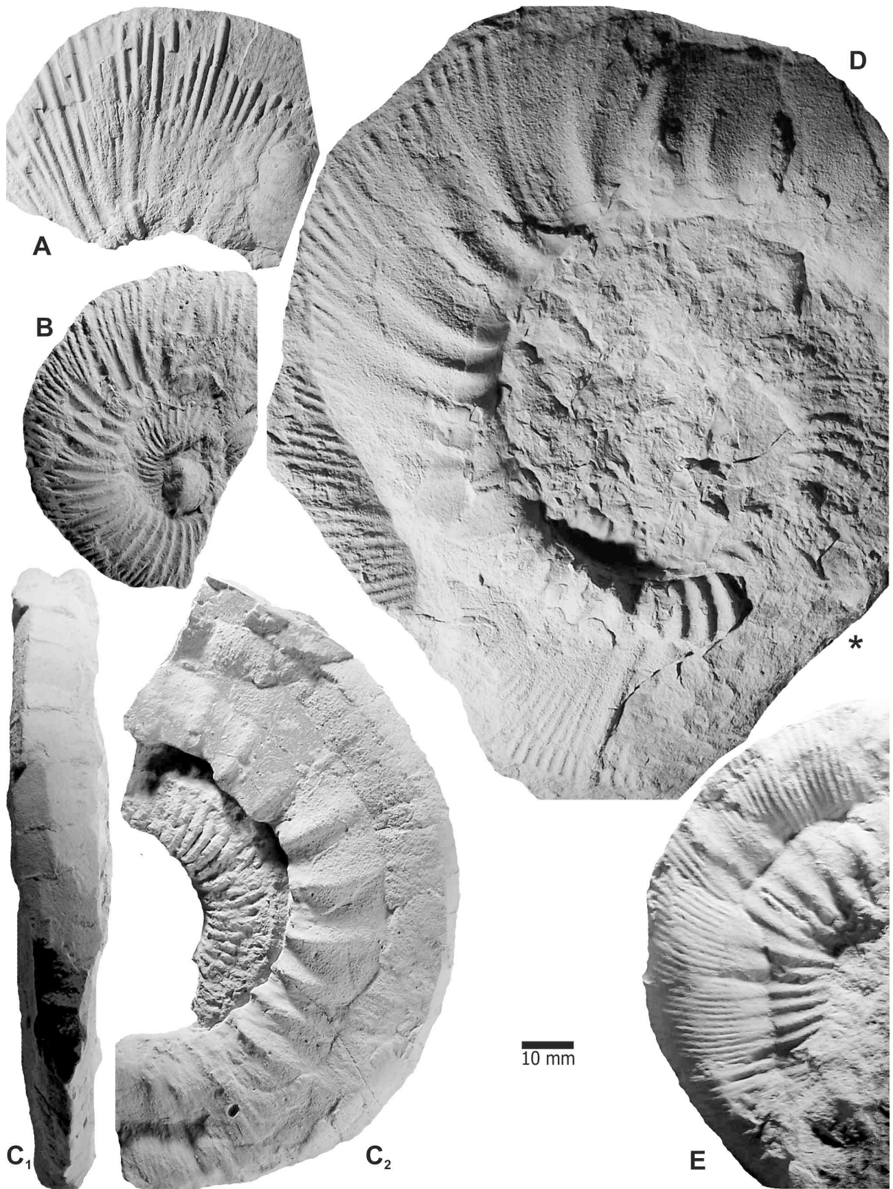
Figure 6. A-B: Choicensisphinctes platyconus Parent, Garrido, Schweigert & Scherzinger, Arroyo Cieneguita, bed AC-1 (Picunleufuense Z., picunleufuense \alpha lz.); A: fragmentary phragmocone (MCNAM 2436); B: fragmentary bodychamber (MCNAM 24366). C-E: Choicensisphinctes cf./aff. platyconus Parent, Garrido, Schweigert & Scherzinger, A. Cieneguita, bed AC-2 (Picunleufuense Z.); C: adult macroconch bodychamber with remains of phragmocone (MCNAM 24367); D: adult macroconch (MCNAM 24370/1) with almost complete bodychamber; E: portion of adult phragmocone (MCNAM 24368). All natural size. The asterisk indicates the last septum.
