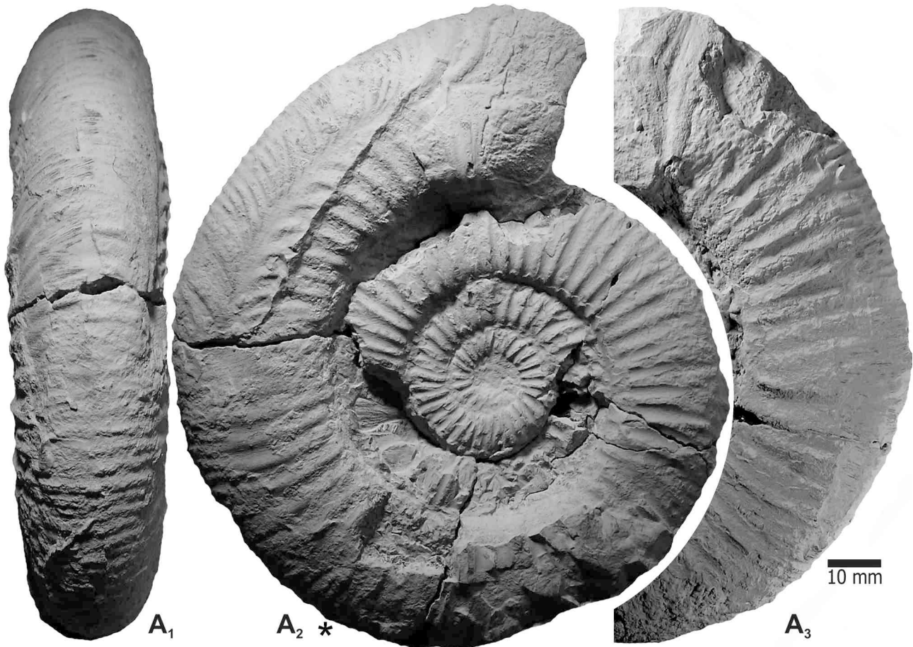
Figure 4. Lithoceras n. sp. aff. picunleufuense Parent, Garrido, Schweigert & Scherzinger. Arroyo Cieneguita, bed AC-6 (Proximus Z.). Adult microconch with lappets (MCNAM 24395). A 1 : ventral view; A 2 : lateral view showing a repaired injury in the left flank (frontal apertural view) not affecting the venter; A 3 : lappet preserved on the right flank. Natural size. Asterisk indicates the last septum.
