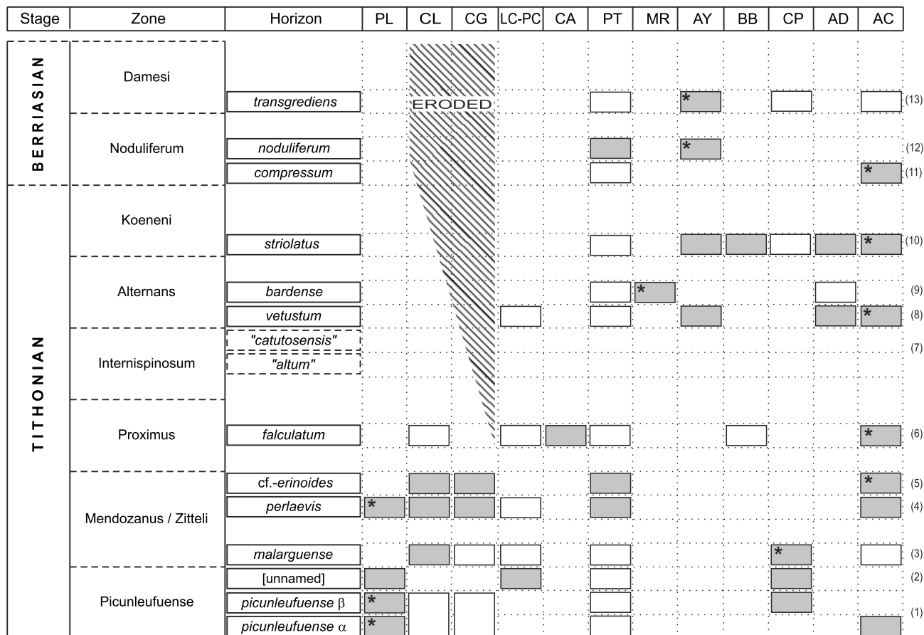
Figure 40. Regional biostratigraphic time-correlation chart for the Neuquén-Mendoza Basin. Correlations based on the recognition of ammonite horizons through the transect of selected localities indicated in Fig. 1 (see abbreviations). The height of the boxes of each zone does not indicate time-duration neither content of horizons, they are sized for convenience of design. Firm recognition of horizons indicated with gray boxes, tentative with white boxes. The asterisk indicates the type locality or section. The Mendozaanus and Zitteli zones are not separated because the impossibility of discrimination in AC and other studied localities (see discussion in text and in PGSS 2011). In most localities several levels with ammonites are known between the horizons indicated in this figure, but they are not indicated because they have not been evaluated for the adjustment to the criteria used in this study. The height of the horizon within each zone is arbitrary for other horizons could be established above and/or below (see details in text). Notes: (1): the picunleufuense α hz. and picunleufuense β hz. were defined in Picún Leufú and their recognition in other localities was already discussed (PGSS 2011). The picunleufuense α hz. is the base of the Picunleufuense Standard Zone. Abundant material of these two horizons was recently collected in PT. These horizons were defined in the southernmost portion of the NMB, their recognition in AC (northern part of the basin) and in several other intermediate localities indicates the horizon is a reliable marker for regional time-correlation. In LA-CG and CL both horizons occur undifferentiated in a basal conglomerate of the Vaca Muerta Fm. (2): this horizon is characterized by a conspicuous new species described preliminary as Choicensisphinctes cf./aff. platyconus (see Fig. 6C-E and PGSS 2011: fig. 23B-E), very close to C. platyconus and C. burckhardtii . In CP a good specimen was figured in Parent (2003: fig. 8) as C. choicensis . In AC it corresponds to bed AC-2. (3): the malarguense hz. has its type locality at CP (PGSS 2011). In PC could be represented by ammonites collected in the upper part of the bed PC-2 of the section described in Parent & Cocca (2007). (4): the perlaevis hz. (defined in PGSS 2011) was recently recognized in CL and CG and is represented by the bed AC-4. In PT the horizon is well represented by C. perlaevis abundant, P. zitteli , small Physodoceras and the same morphotype of Choicensisphinctes cf. erinoides than in PL. (5): the guide-assemblage of the cf. erinoides hz. includes specimens similar to the type specimens of C. erinoides , C. australis and C. mendozanus from Cajón del Burro-Río Choicas (Burckhardt 1900), suggesting very similar age with the guide-assemblage of the Mendozaanus Z. of Burckhardt (1903: 106). The type horizon of C. limits at Paso Montañas includes a specimen (Burckhardt 1900: pl. 25: 2) similar to C. cf. guenakenensis described above from bed AC-4 ( perlaevis hz.). (6): the falculatum hz. introduced in this report yields a rich ammonite assemblage. In a thick succession of beds in CL-CG there occur a very abundant and rich fauna including P. subpretiosus , C. falculatum , C. proximus and Toulisphinctes rafaeli . This assemblage indicates very closely the falculatum hz., but the fauna is very abundant and probably after description could be discriminated different new ammonite horizons within the Proximus Z. which are commonly not recorded in the successions of southern Mendoza. (7): the "altum" and "catutosensis" horizons [after Aspidoceras altum Biró, 1980 and Catutosphinctes catutosensis (Leanza & Zeiss, 1990)] were introduced by Leanza & Zeiss (1992) for the Internispinosum Z. of the local succession of Los Catutos. Nevertheless, only three ammonite impressions were illustrated what prevents their use for comparison, and, on the other hand, similar ammonites are known from CL and LC but in different stratigraphic positions. For the time being these two horizons are not considered for correlation. (8): the vetustum hz. is recognized in AD (very close to AC) on the basis of the ammonite assemblage listed by Krantz (1928: 49), including different morphotypes of C. mendozanum as described above, Blanfordiceras argentinum , B. vetustum (as Berriasella subprivasensis ), P. calistoides and A. andinum Steuer, 1897. The beds with these ammonites were denominated the "Berriasella calistoides Zone" by Krantz (1928: 49), which should be equivalent to the vetustum hz. In AY, the bed c of Leanza (1945: 89) yields Corongoceras mendozanum (as Aulacosphinctes sp., discussed above, under C. mendozanum ) and Catutosphinctes australis (Leanza, 1945) which is indistinguishable from C. inflatus of the vetustum hz. (9): the type horizon of S. alternans , bed 31 g of the section of AD (Gerth 1925: 126), comprises ammonites very similar to those of the guide assemblage of the bardense hz. from MR, but it also includes S. koeneni and the range of variation of S. alternans is different as described in text. (10): the striolatus hz. is represented in AY by the bed f of Leanza (1945), in BB (Krantz 1928, Gerth 1925: 122) and in AD by the bed 31h (in Gerth 1925: 126, see discussion in text). In CP the specimens of C. striolatus (see Parent 2003) are similar to those of AC but the other species of the guide assemblage are not recorded. (11): the compressum hz. could be present in PT by the occurrence of the index in abundance but only microconch Spiticeras were collected that remain to be studied. (12): the noduliferum hz. could be used conveniently for standardization of the Noduliferum Z. For the time being it has been clearly recognized in PT. (13): the transgrediens hz. could be used conveniently for standardization of the Damesi Z. In CP (Parent 2003) have been collected few well preserved specimens almost identical with the HT (by MT) of Cuyaniceras transgrediens from the bed 6 of Gerth (1925: fig. 15).
