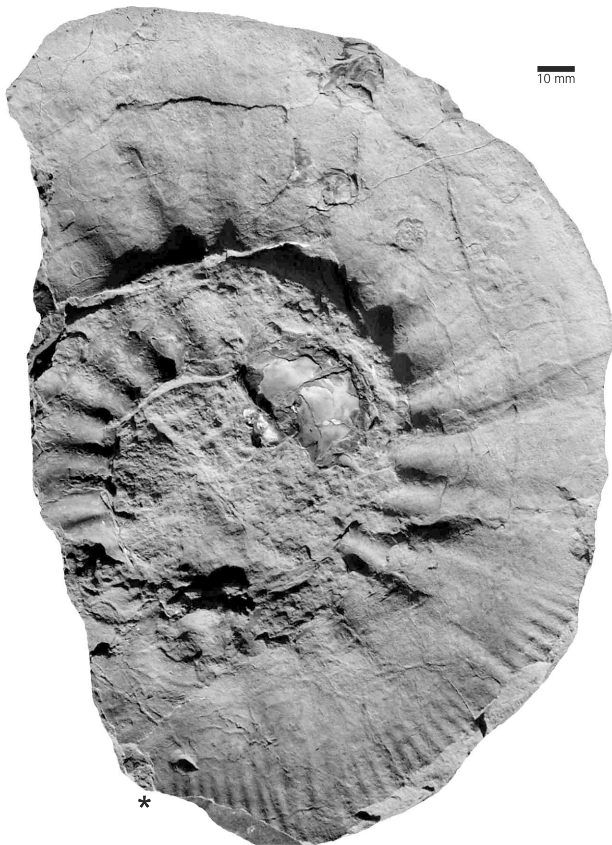
Figure 9. Choicensisphinctes cf. erinoides (Burckhardt). Almost complete adult macroconch of an evolute variant (negative field-photograph of a cast, natural size). Arroyo Cieneguita, bed AC-5 (Zitteli Z., cf. erinoides hz.). Natural size. Asterisk indicates the last septum.
