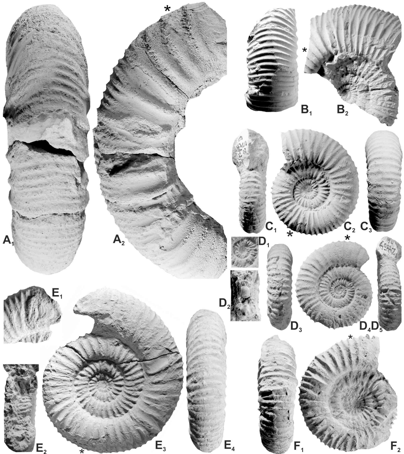
Figure 18. Catutosphinctes proximus (Steuer), A. Cieneguita, Proximus Zone. A: half whorl of macroconch phragmocone with beginning of bodychamber (MCNAM 24466), bed AC-7. B: macroconch phragmocone with portion of bodychamber (MCNAM 24412), bed AC-7. C: almost complete adult microconch (MCNAM 24459/25), involute-stout variant, bed AC-8. D: adult microconch phragmocone with beginning of bodychamber (24459/26), compressed-evolute variant, bed AC-8; D 1 -D 5 : lateral and ventral views of innermost whorls (x2). E: complete adult microconch with lappets (MCNAM 24439), bed AC-7; E 1 : detail of the lappet, left face apertural view; E 2 : detail of inner whorl showing continuous ribbing through the venter. F: adult microconch with a quarter whorl of bodychamber (MCNAM 24445), bed AC-7. All natural size otherwise indicated. Asterisks indicating the last septum.
