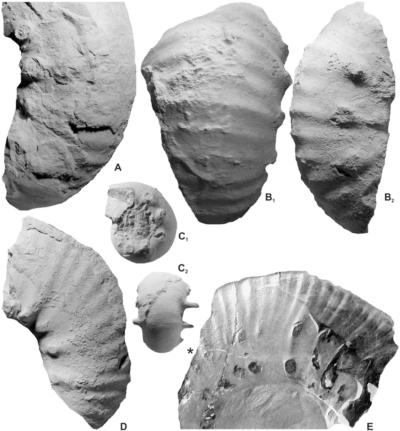
Figure 36. A-C: Aspidoceras cf. euomphalum Steuer, A. Cieneguita; A: portion of macroconch bodychamber (MCNAM 24424), bed AC-7 (Proximus Z., falculatum Hz.) with test preserved showing the tubercles of internal mold below hollow spines with subcircular base; B: portion of macroconch bodychamber (MCNAM 24415/7), bed AC-7; C: juvenil macroconch phragmocone (MCNAM 24456/2), bed AC-11 (Internispinosum Z.) with test preserved showing the tubercles of internal mold below long spatulate, hollow spines with subcircular base. D-E: Toulisphinctes cf. rafaeli (Oppel), A. Cieneguita; D: portion of macroconch phragmocone (MCNAM 24418/1), bed AC-8 (Proximus Z.); E: adult macroconch bodychamber with terminal portion of phragmocone (negative field-photograph of a cast not collected, x0.5), bed AC-7. All natural size otherwise indicated. Asterisks at last septum.
