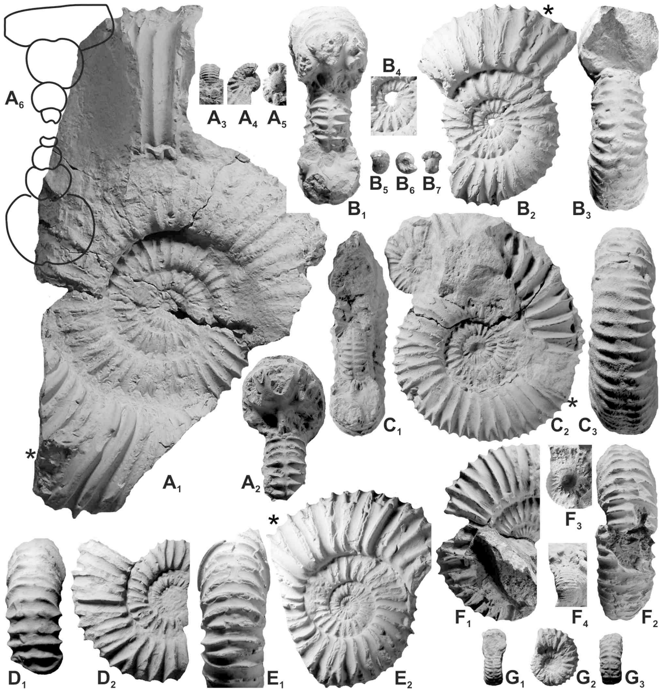
Figure 21. Catuosphinctes inflatus (Leanza, 1945). A. Cieneguita, beds AC-15 (Alternans Z., vetustum hz.) and AC-16 (Alternans Z.). A: complete adult macroconch (MCNAM 24460/2, bed AC-16), showing the venter of juvenil phragmocone ( A 2 ) and innermost whorls at the onset of lateral ribbing and slightly later the ventral ribbing ( A 3 -A 5 , x2); A 6 : whorl section at about D = 80 mm. B: adult microconch? phragmocone with the beginning of the bodychamber (MCNAM 24457/8, bed AC-15), showing venter of juvenil phragmocone ( B 1 ), inner whorls ( B 4 , x2) and innermost whorls (detached) at the onset of lateral ribbing ( B 5 -B 7 , x2). C: juvenil macroconch with incomplete bodychamber (MCNAM 24457/6), bed AC-15, showing the venter of the juvenil phragmocone ( C 1 ). D: adult microconch? phragmocone (MCNAM 24460/3), bed AC-16. E: adult microconch? with incomplete bodychamber (MCNAM 24457/8), bed AC-16. F: adult microconch? phragmocone (MCNAM 24460/1), bed AC-16, showing the inner whorls densely ribbed ( F 1 -F 4 , x2). G: juvenil specimen (MCNAM 24457/20), bed AC-15, with beginning of bodychamber. All natural size otherwise indicated. The asterisks indicate the position of the last septum.
