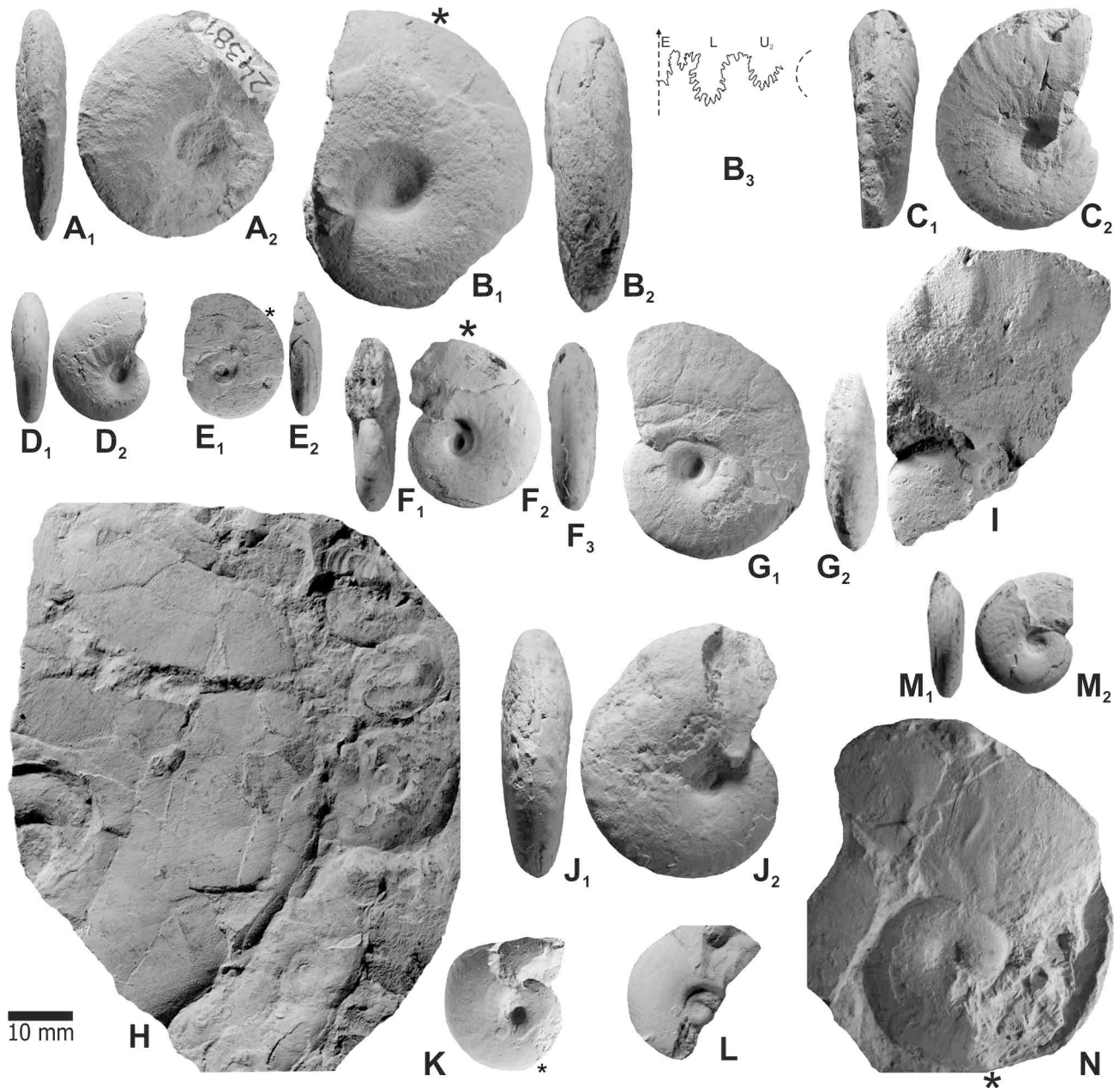
Figure 39. A: Pasottia andina Parent, Schweigert, Scherzinger & Enay, macroconch phragmocone (MCNAM 24381), bed AC-4 (Mendozanus-Zitteli zones). B: Pseudolissoceras zittelli (Burckhardt), adult macroconch with a portion of bodychamber (MCNAM 24375), bed AC-5 (Zitteli Zone); B 3 : septal suture line(x1) at D = 41 mm. C: Parastreblites? cf. comahuensis Leanza, phragmocone (MCNAM 24399), bed AC-4 (Zitteli Zone). D: Semiformiceras? sp. A, phragmocone (MCNAM 24405), bed AC-5 (Zitteli Zone). E: Uhligites? sp. A, adult specimen with a quarter whorl bodychamber (MCNAM 24406/2), bed AC-8 (Proximus Zone). F: Cieneguiticeras? sp. A., apparently adult phragmocone with beginning of the bodychamber (MCNAM 24399/1), bed AC-5 (Zitteli Zone). G-H: Cieneguiticeras perlaevis (Steuer), A. Cieneguita; G: juvenil macroconch with beginning of bodychamber (MCNAM 24377), bed AC-5 (Zitteli Zone); H: adult macroconch and adult microconchs (MCNAM 24370/2) associated in a concretion with Choicensisphinctes cf./aff. platyconus (MCNAM 24370/1 in Fig. 6D), bed AC-2 (Picunleufuense Zone). I-N: Cieneguiticeras falculatum (Steuer), bed AC-7 (Proximus Zone, falculatum hz.); I: adult macroconch (MCNAM 24404/6); J: macroconch phragmocone (MCNAM 24405); K: adult microconch (MCNAM 24404/10); L: adult microconch (MCNAM 24404/7); M: adult microconch (MCNAM 24407/4) with most part of bodychamber; N: almost complete adult macroconch (MCNAM 24404/15). All specimens from Arroyo Cieneguita. All natural size. Asterisk indicating the last septum.
