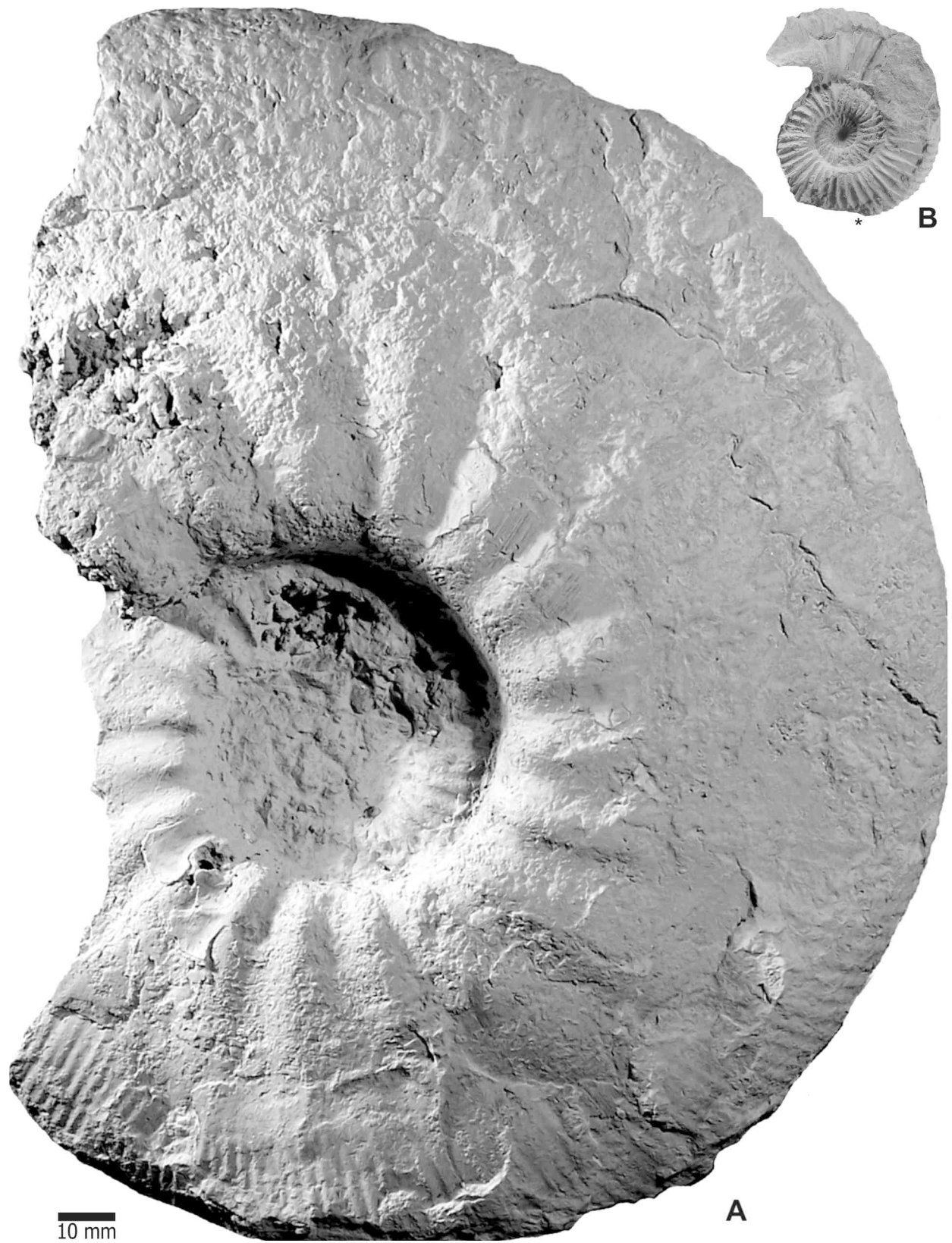
Figure 13. A: Choicensisphinctes cf. limitis (Burckhardt), crushed adult phragmocone (MCNAM 24388), Arroyo Cieneguita, bed AC-5 (Zitteli Z., cf. erinooides hz.). B: Choicensisphinctes sp. A, complete adult microconch with lappets (MCNAM 24445/2), A. Cieneguita, bed AC-7 (Proximus Z., falculatum hz.). All natural size. Asterisk indicating the last septum.
