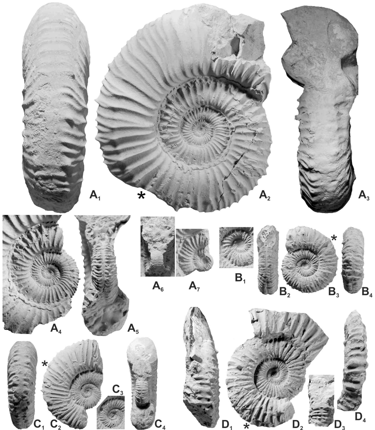
Figure 30. Steueria alternans (Gerth, 1921), A. Cieneguita, beds AC-14 (A) and AC-15 (B-D), Alternans Zone. A: almost complete adult macroconch (MCNAM 24402), showing details of the inner whorls (A 4 -A 7 , x2). B: juvenil specimen with beginning of bodychamber (MCNAM 24459/X2), B 1 : details of the innermost whorls (x2). C: juvenil specimen with beginning of bodychamber (MCNAM 24459/X1), C 1 : details of the innermost whorls (x2). D: subadult macroconch with almost complete bodychamber (MCNAM 24459/19); D 1 : ventral view of the last whorl of the phragmocone, D 2 : lateral view, D 3 : ventral view at the beginning of the bodychamber, D 4 : ventral view of the last preserved part of the bodychamber. All natural size otherwise indicated. Asterisks indicating the last septum.
