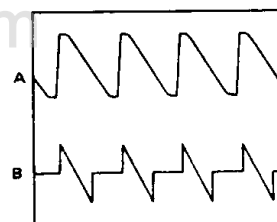
Figure 9. Sinusoidal Sawtooth and Linear Ramp Outputs
