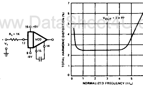
Figure 8. Sinusoidal Output Distortion as a Function of Frequency Sweep
