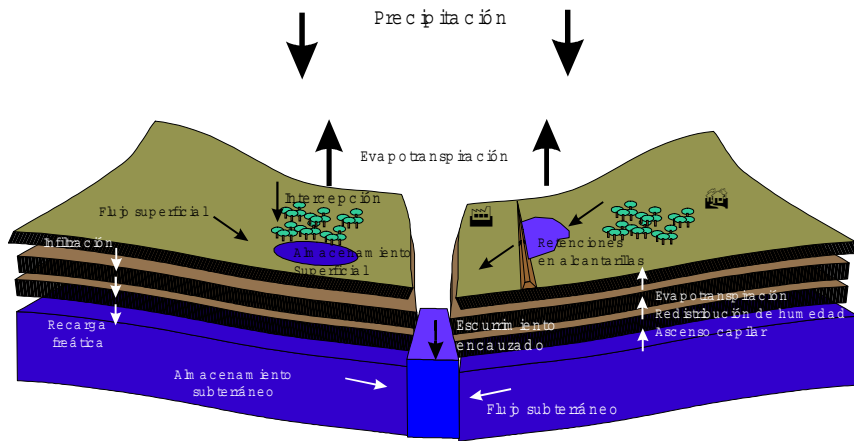
Figure 1 Scheme of assemble between surface, unsaturated and gronwater cells
