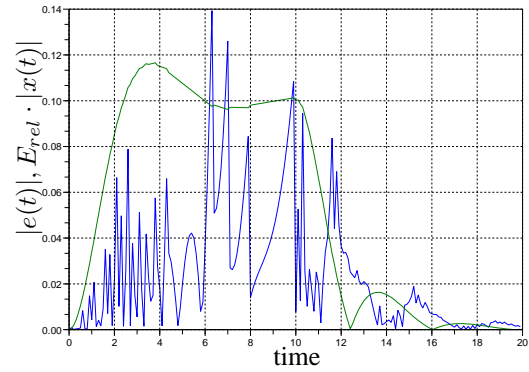
Figure 4: Absolute error
