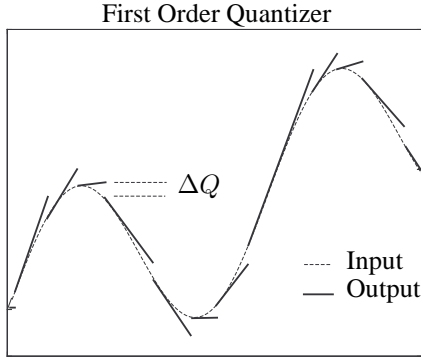
Figure 2: Trajectories of a first-order quantizer.
