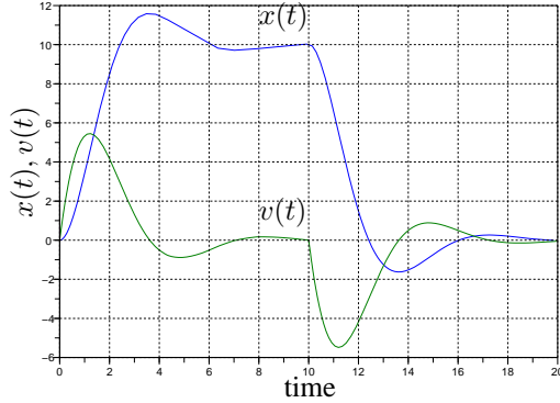
Figure 3: Spring–Mass System Trajectories
