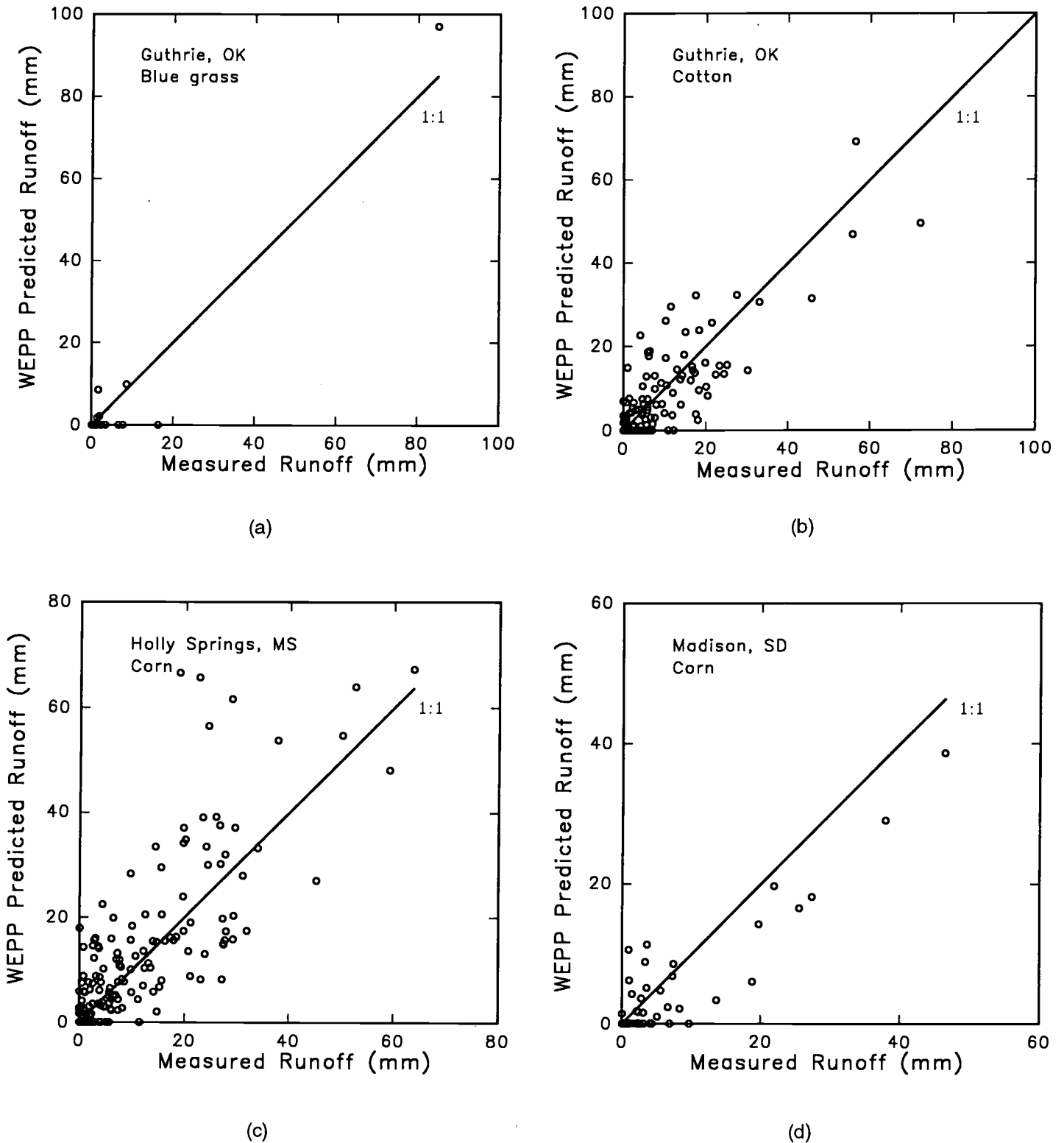
Figure 6. Measured Versus WEPP-Predicted Individual Storm Runoff Volume for Cropped Conditions Using Effective Hydraulic Conductivity Values, K_e , Estimated Using Relationships from Table 8 for Data from: (A) Guthrie, Oklahoma, for Blue Grass; (B) Guthrie, Oklahoma, for Cotton; (C) Holly Springs, Mississippi, for Corn; and (D) Madison, South Dakota, for Corn.
